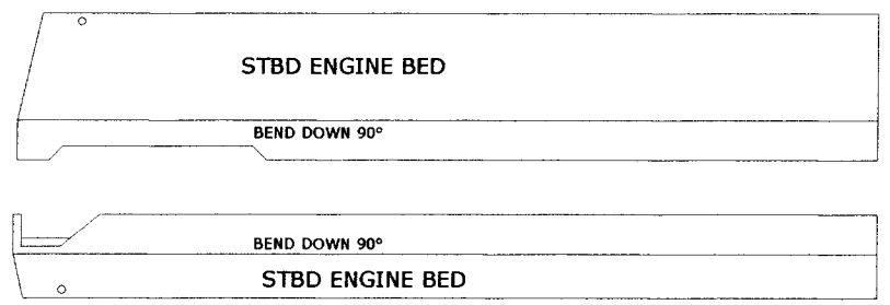
ENGINE BEDS COPIED (NOT MIRRORED)
