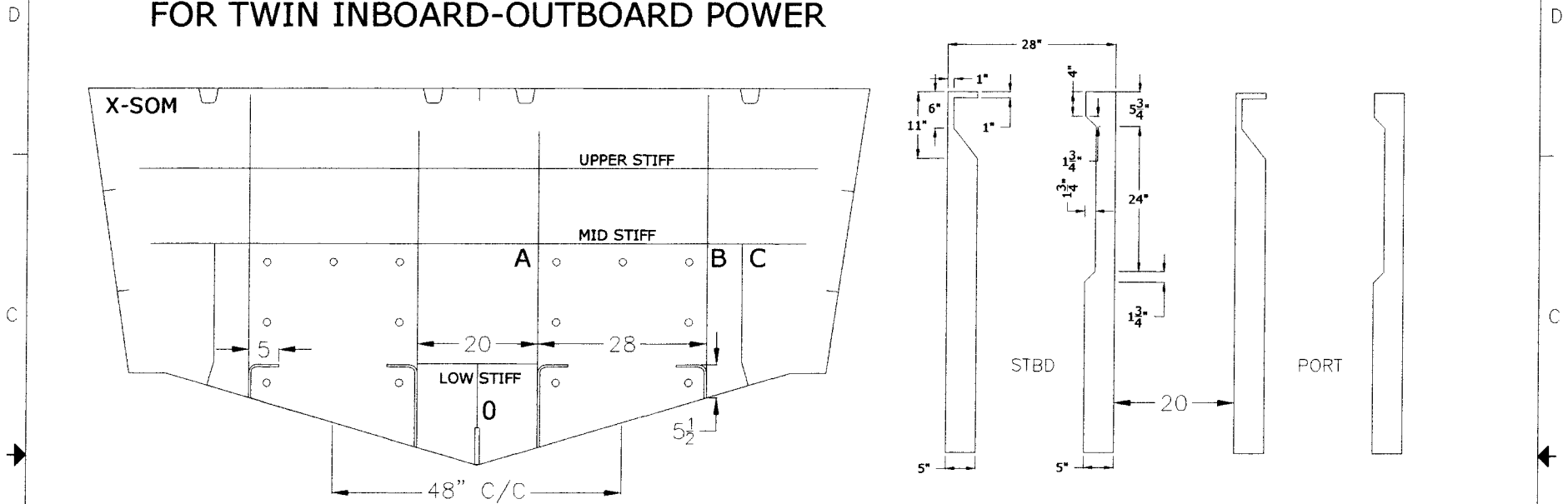
ENGINE BEDS COPIED (NOT MIRRORED)
