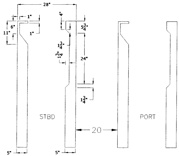
ENGINE BEDS COPIED (NOT MIRRORED)
