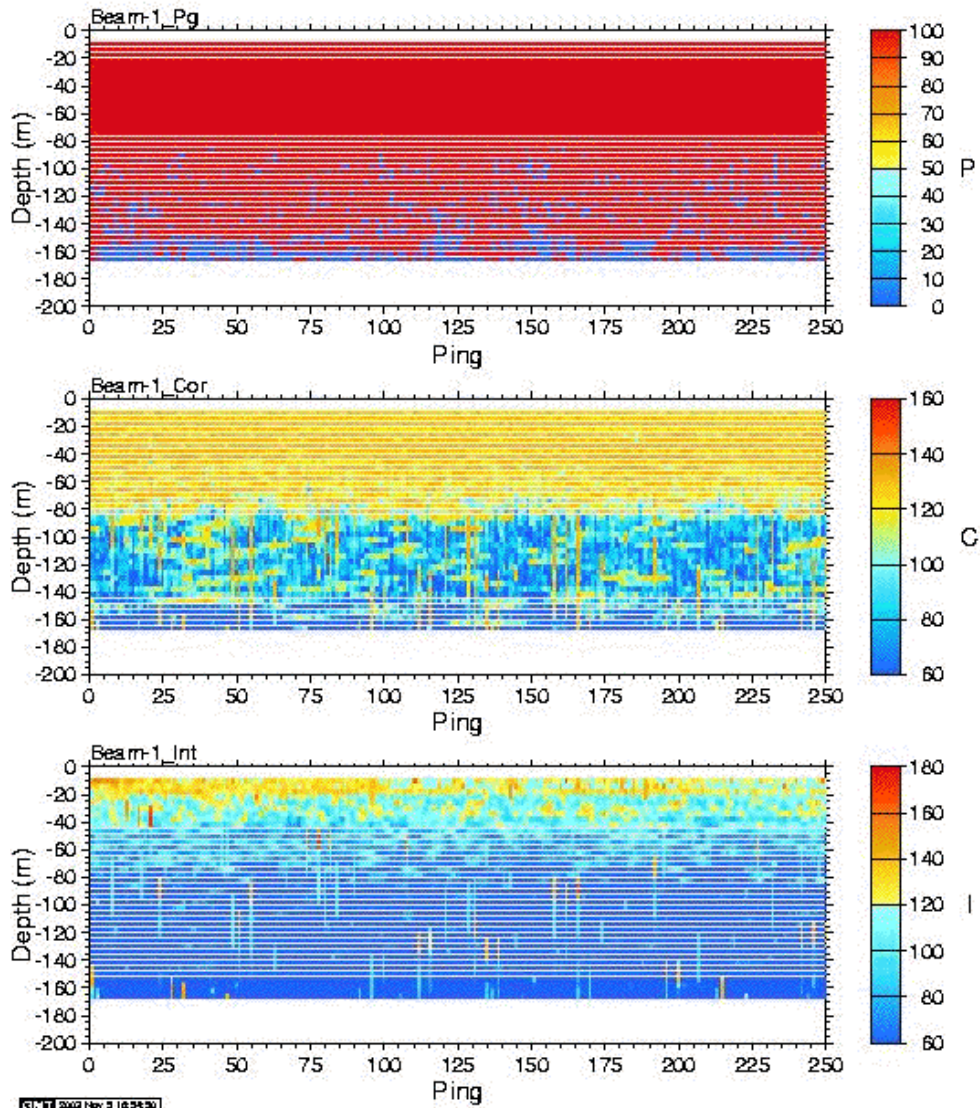
Fig. 4: Time-series of “%-good-pings” (top), “correlation” (middle), and “echo intensity” (bottom) for 250 single pings of beam-1 while the ship is on station in water >1000-m deep in the Beaufort Sea (Oct.-03, 2003, ~05:30 UTC).
