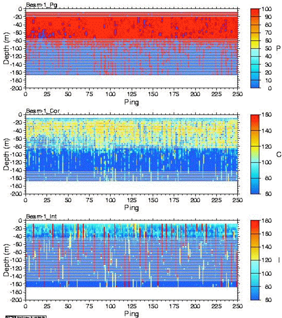
Fig. 8: As Fig. 4, but while the ship is steaming at ~10 kts in water >300-m (Sept.-24, 2003, ~03:55 UTC). Note the large echo intensity (bottom panel) that occurs intermittently throughout the entire water column. It corresponds to low correlation (middle panel) and often is flagged falsely as a good ping (top panel). This erroneous signal originates from within the ship.
